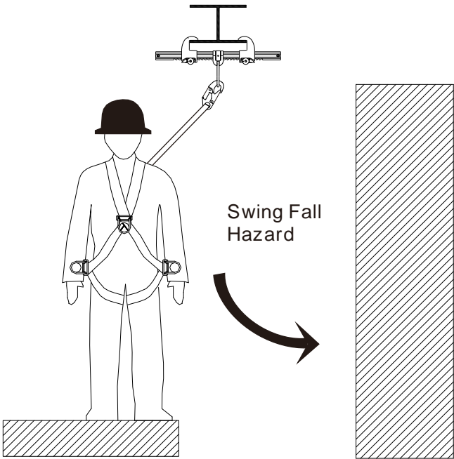
Swing Falls
